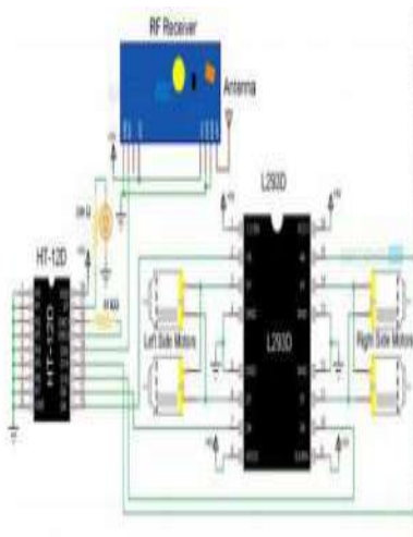
Fig 4. Receiver
