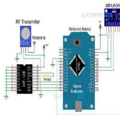
Fig 3. Transmitter
