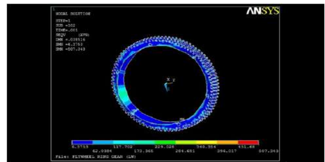
Fig. 7.4: Stress Analysis of FLYWHEEL RING GEAR
