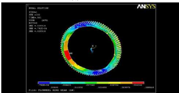
Fig. 7.2: Displacement of FLYWHEEL RING GEAR
