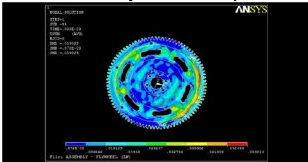
Fig. 7.1: Displacement of FLYWHEEL ASSEMBLY
