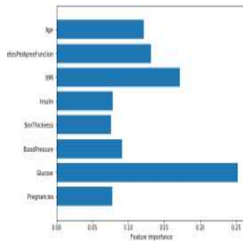
Figure 4: Feature Importance Plot for Random Forest
