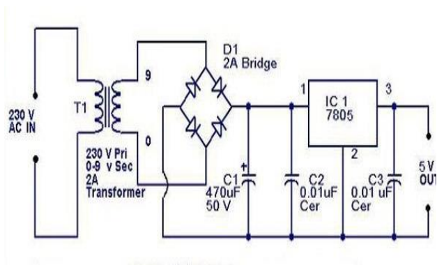
Fig. 3.2: Circuit diagram of regulated power supply section
