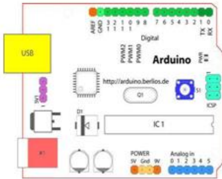
Figure 3.3 Structure of Arduino Board
