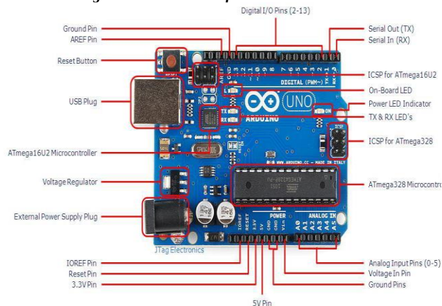
Figure3.4 Arduino Board
