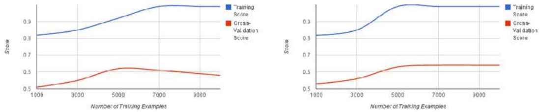
Figure 3. Training curve for GLM models. (Left: Raw, Right: PCA)
