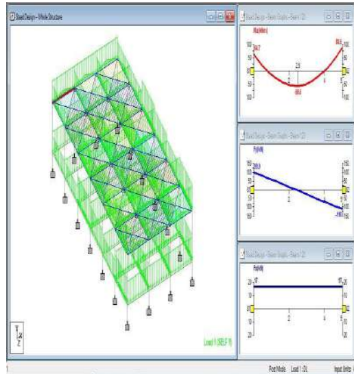
Fig. 2.1.7 VIEW OF LOAD 1(SELF Y)
