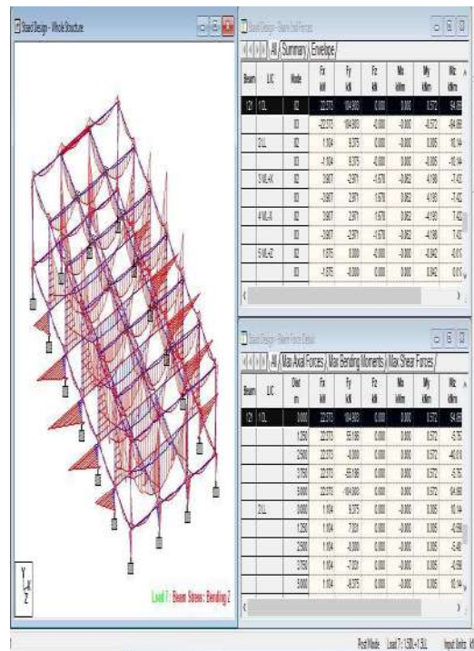
Fig. 2.1.7 VIEW OF LOAD 1(SELF Y)
