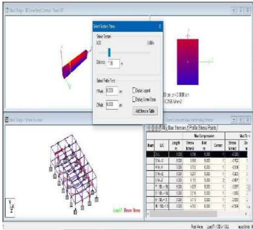
Fig. 2.2.1 BEAM STRESS
