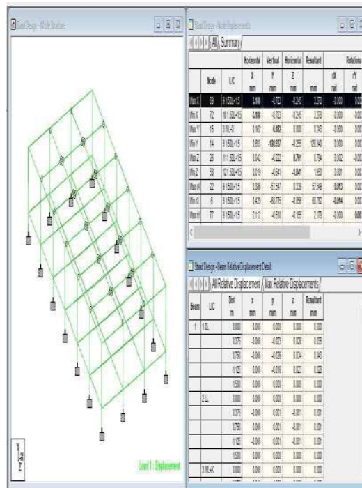
Fig.2.1.6 DISPLACEMENT VIEW
