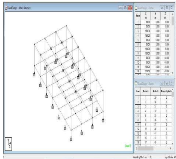
Fig. 2.1.3 STRUCTURE VIEW
