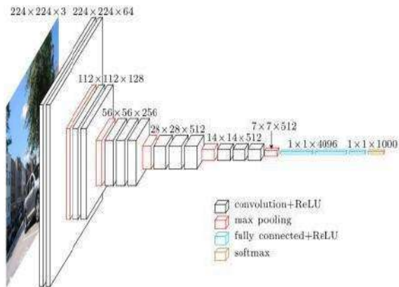
Fig.1: CNN Architecture
