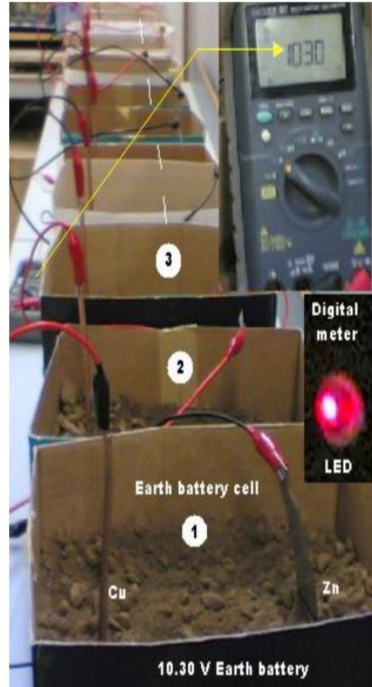
a. A twelve cells 10.30V/45mA earth battery
