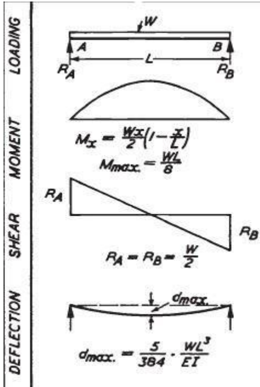
Fig -3: simply supported beams - UDL as per Steel Designer's Manual - AISI
