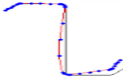
Fig 9 (a): LOCAL BUCKLING Beam deflects laterally Fig 9 (b): DISTORSIONAL BUCKLING Beam twists and deflects laterally
