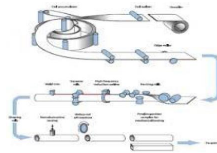
Fig-1: Linediagram showing cold formed steel processing
