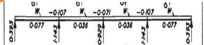
Fig -4 Bending Moment and reaction Co-efficient- Equal span continuous beams - UDL as per Steel Designer's Manual - AISI
