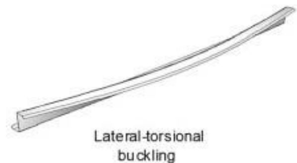
Fig -10: Lateral torsional buckling of Z section
