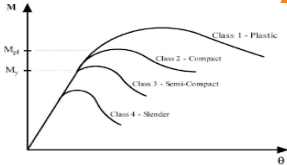
Fig - 2: Graph Showing Classification of Sections with respect to moment (M) and curvature (θ) as per IS800:2007
