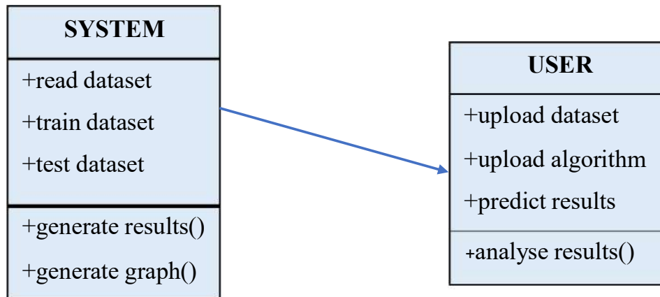
4.1.1 class diagram
