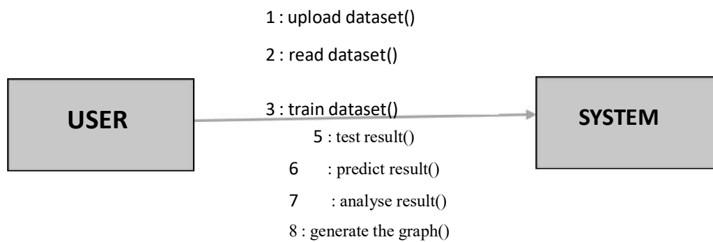
4.1.4 collaboration diagram
