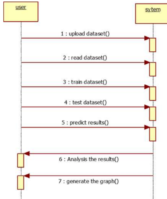
4.1.3 sequence diagram
