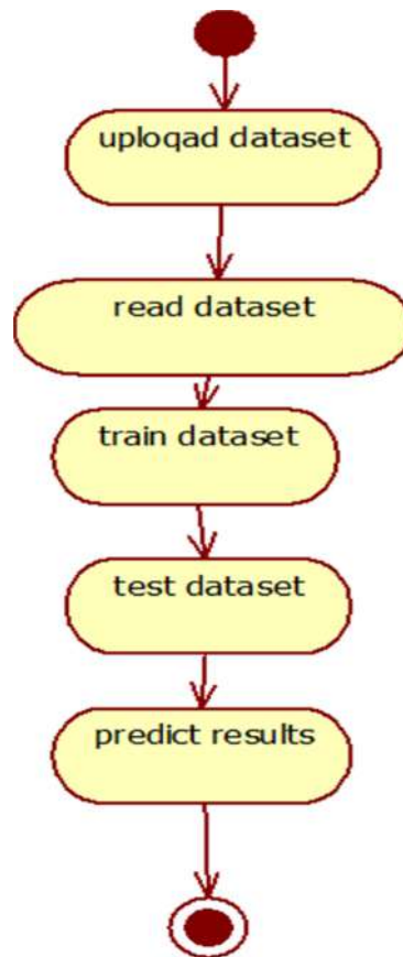
4.1.5 Activity diagram
