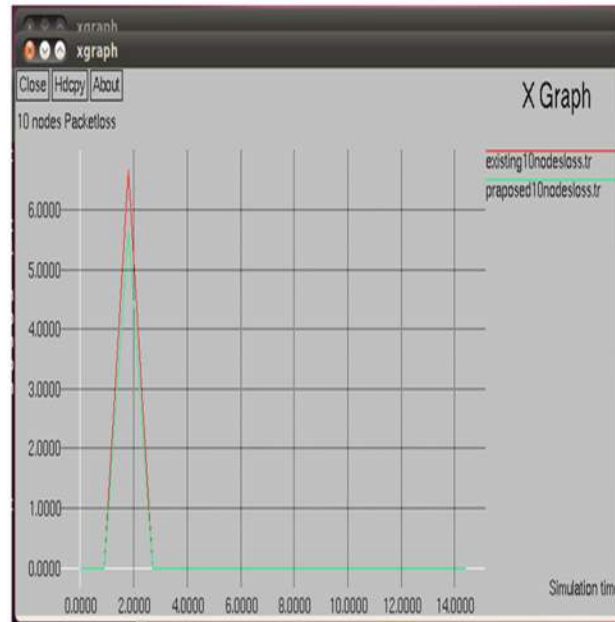
Figure 4.14. Comparison of packet loss number of node (10) with malicious node proposed protocol with existing protocol
