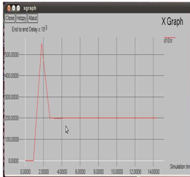
Figure 4.10. Delay of number of node (10) with malicious node proposed protocol
