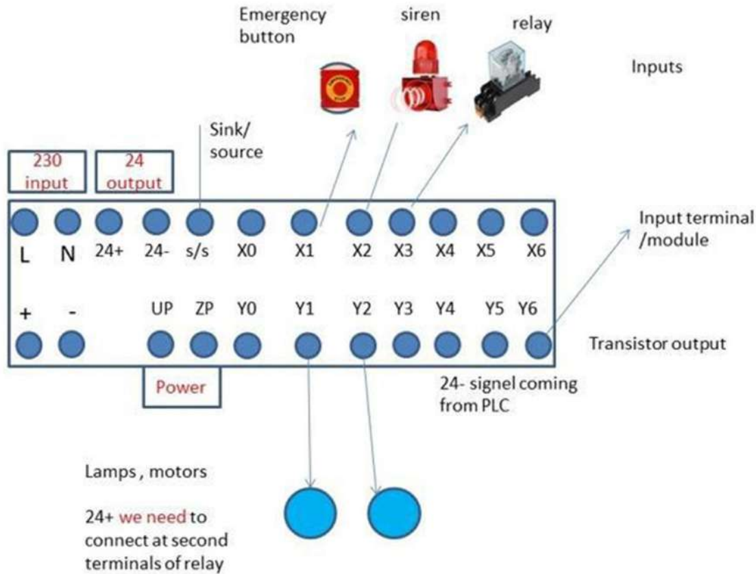
Figure: 6.1.1PLC Project circuit diagram
