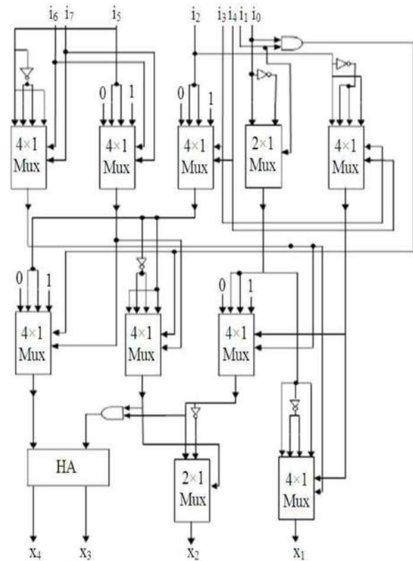
Fig. 4. Implementation of 9- 4 compressor using multiplexer
