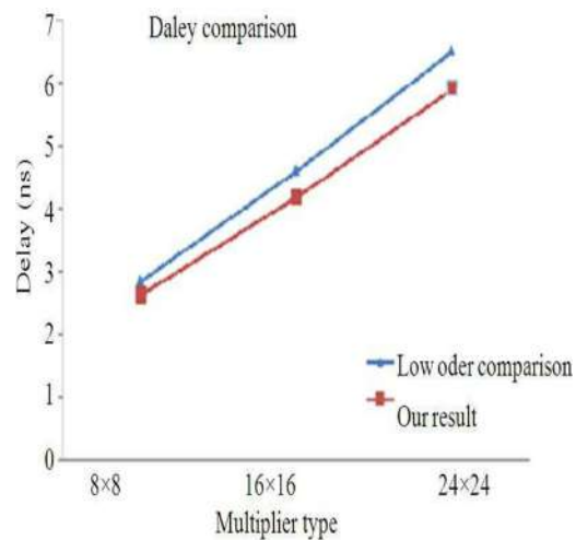
Fig. 6. Speed comparison of different multiplier
