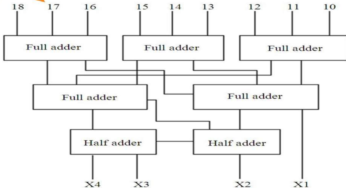
Fig 2 : 9-4 Compressor design
