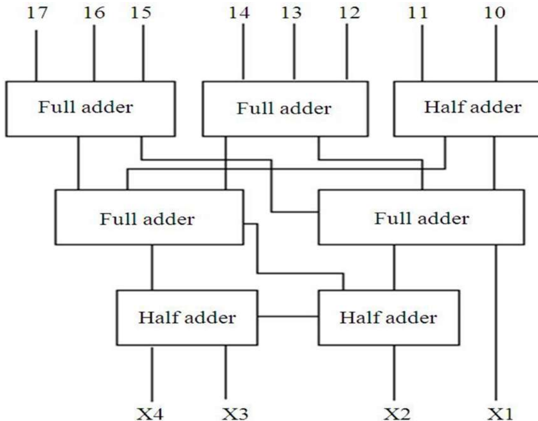
Fig. 1. 8-4 Compressor design
