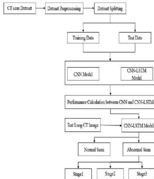
Fig. 3.1 Flowchart of Proposed model
