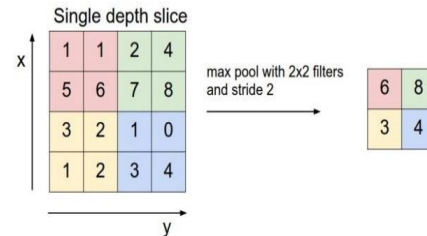
Fig 6: Pooling Layer
